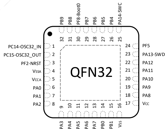
Figure 3-5 QFN32(4*4) PY32F040K3xU7-E Pinout3(Top view)
