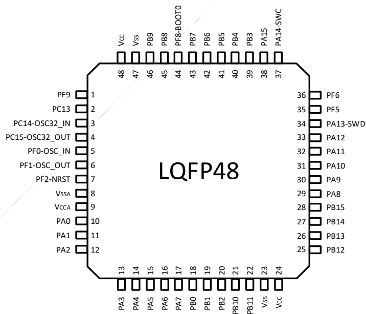
Figure 3-2 LQFP48 PY32F040C1xT7-E Pinout1(Top view)
