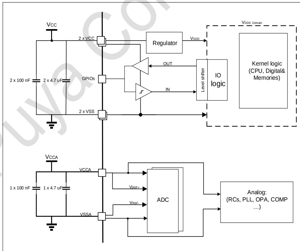
Figure 5-1 Power supply scheme
