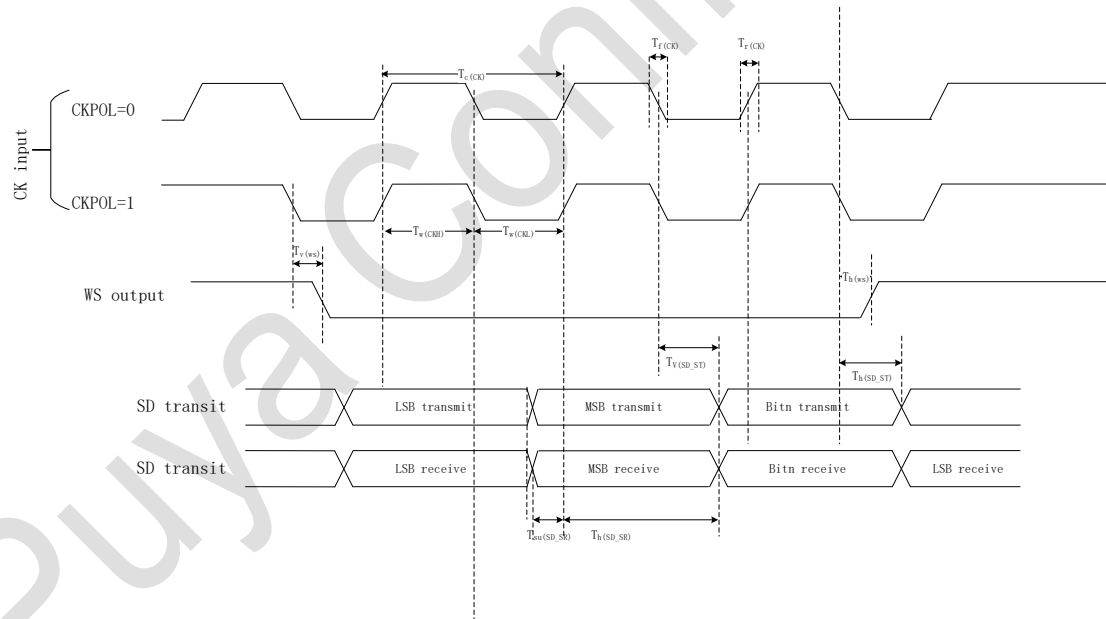
Figure 5-7 I 2 S timing diagram – Master mode(Philips protocol)
