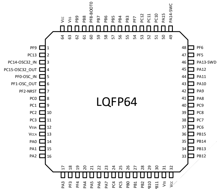
Figure 3-1 LQFP64 PY32F040R1xT7-E Pinout1(Top view)
